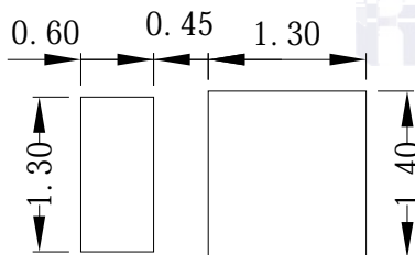
Fig.1-5 Soldering Patterns
