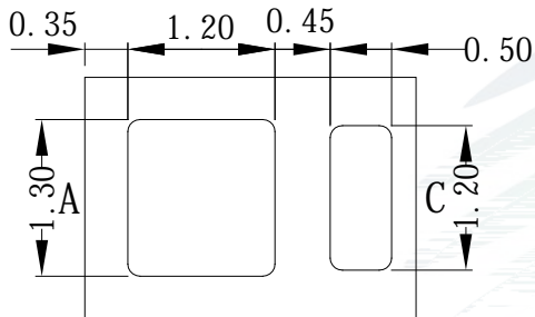
Fig.1-3 Bottom View
