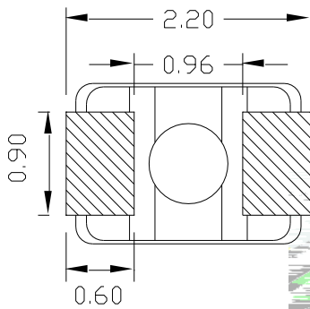
Fig. 1-3 Bottom view
