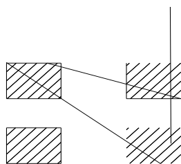
Fig.1-5 Soldering patterns 推荐焊盘
