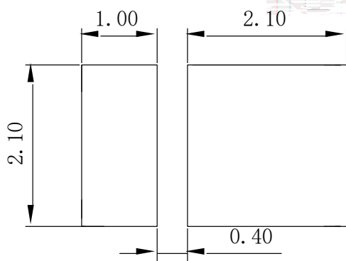
Fig.1-5 Soldering patterns
