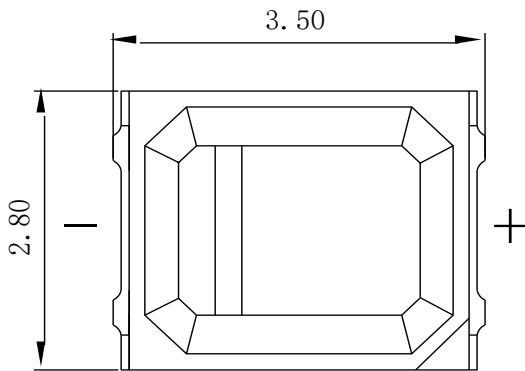
Fig.1-1 Top view
