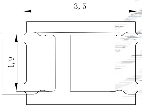
Fig.1-3 Bottom view
