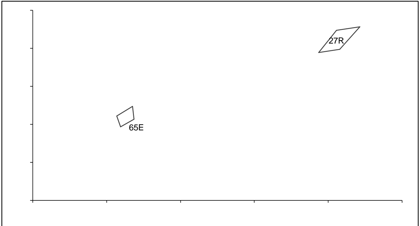
Fig. 1-6 The C.I.E Chromaticity Diagram CIE
